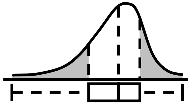
Left-skewed distribution
