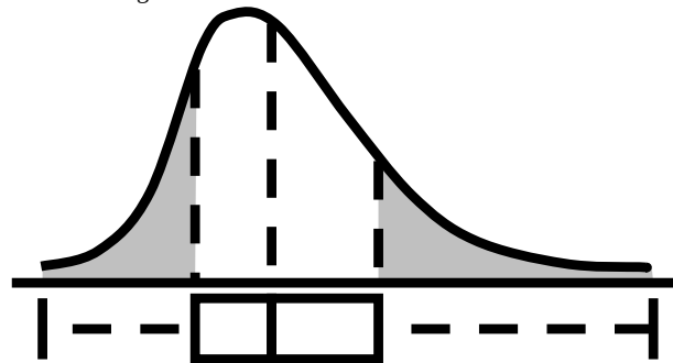
Right-skewed distribution
